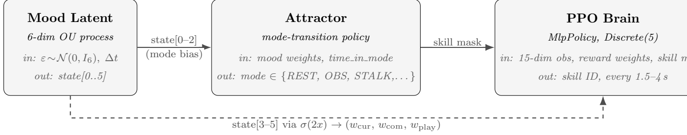
Figure 3: Information flow through the three behavioral components. Solid arrows carry structural information (mode bias, skill mask); the dashed arrow carries mood-modulated reward weights making the PPO’s reward landscape a function of internal state.
