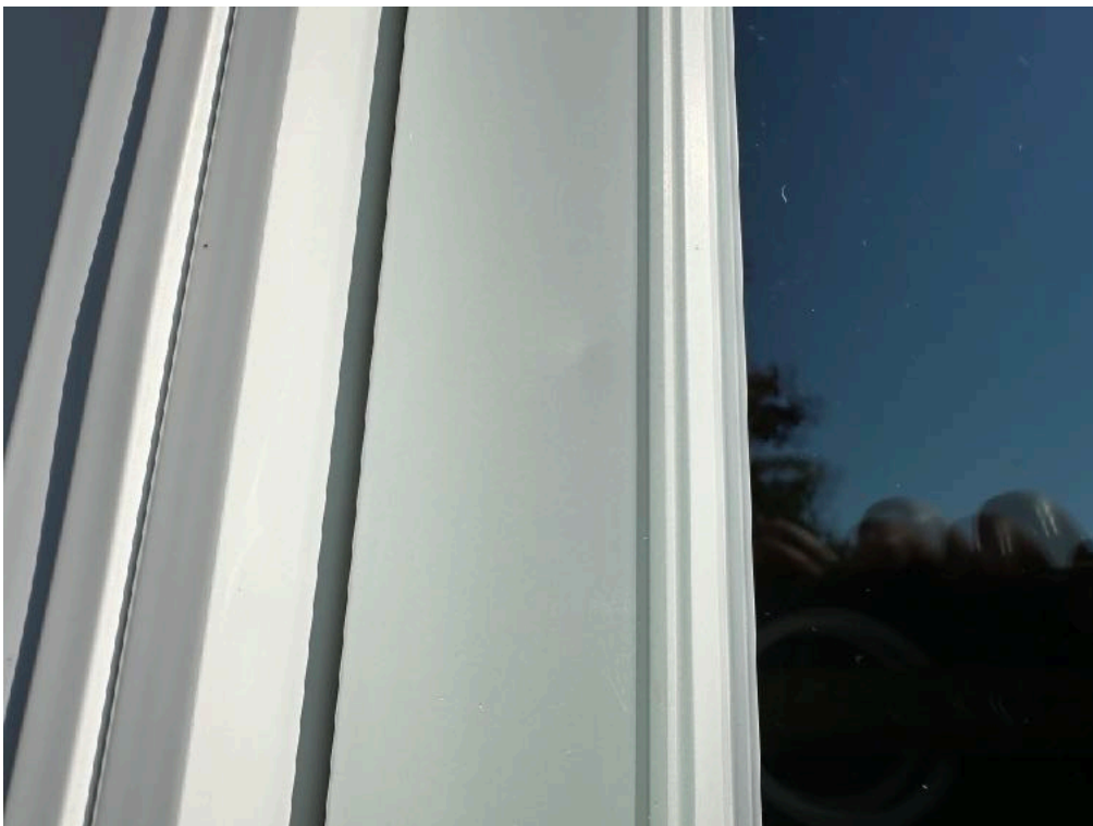
A-40: DENT IN SASH ALONG LEFT SIDE OF CASEMENT
