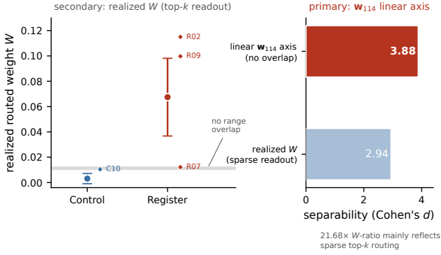
Figure 2: Held-out register/control separability. Left: the separation in realized routed weight W (the secondary, top- k readout; mean \pm sd, n=10 /class, with the named extreme prompts; no range overlap). Right: the primary statistic, the recovered linear w_{114} projection, separates the same split at d=3.88 with no overlap, sharper than realized W . The 21.68\times W -ratio mainly reflects sparse top- k routing, with little added discriminative signal.
