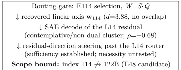
Figure 1: One axis, three readouts, one bound. Routing, SAE semantics, and residual geometry are three readouts of the same E114 register axis; the gate logit is a readout of it, and whether it also controls the register is left open (§8).
