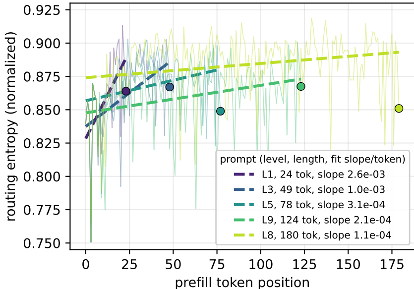
Qwen 397B: routing entropy vs. position
