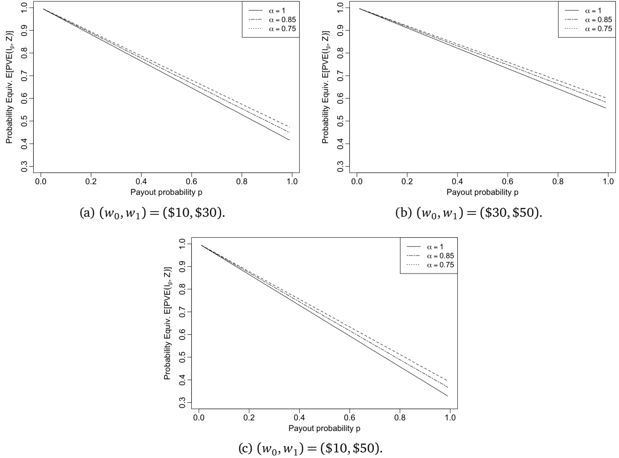
Figure 2: Probability equivalents \mathbb{E}[PE(l_p, Z)] of binary lotteries l_p = (p, w_0, w_1) , where Z consists of yardstick lotteries z^k = (q_k, 0, w_1) . Z is adapted to l_p with |Z| = 15 . \tau has a CDF-complexity representation with u(w) = w^\alpha and H(r) = (\Phi^{-1}(G(r)))^2 , for G given by (1) with \kappa = 0 , \gamma = 0.5 . Priors are distributed Q \sim U[0, 1] .
