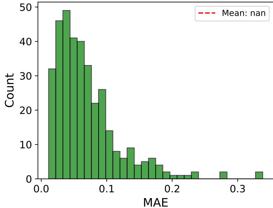
delta_B MAE Distribution
