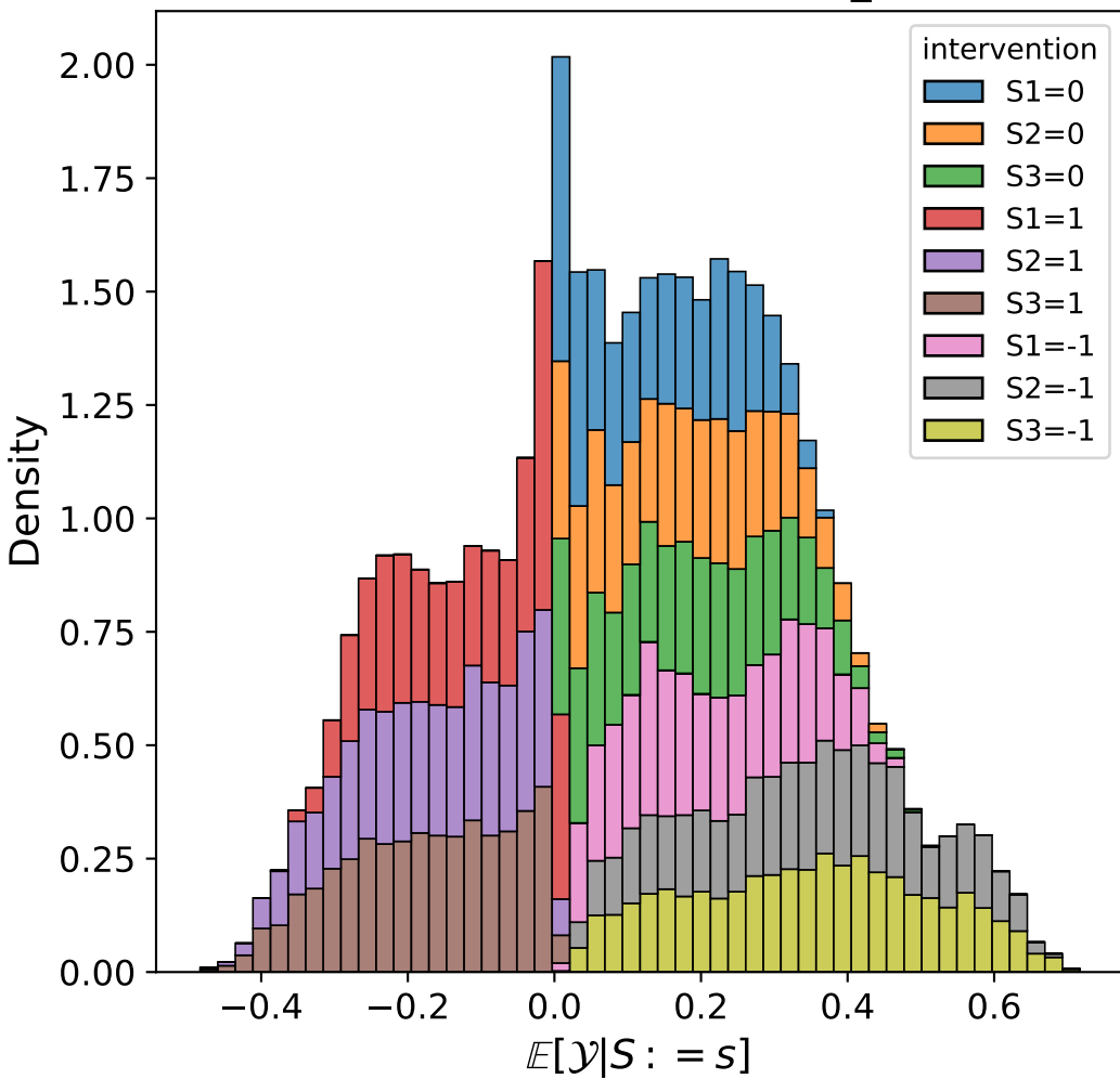
Variable \mathcal{Y} = Y1 , fold=k_0
