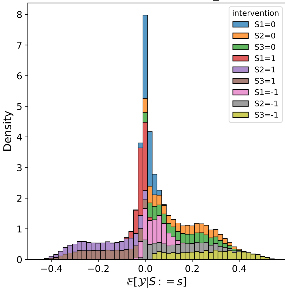
Variable y = Y2 , fold=k_3
