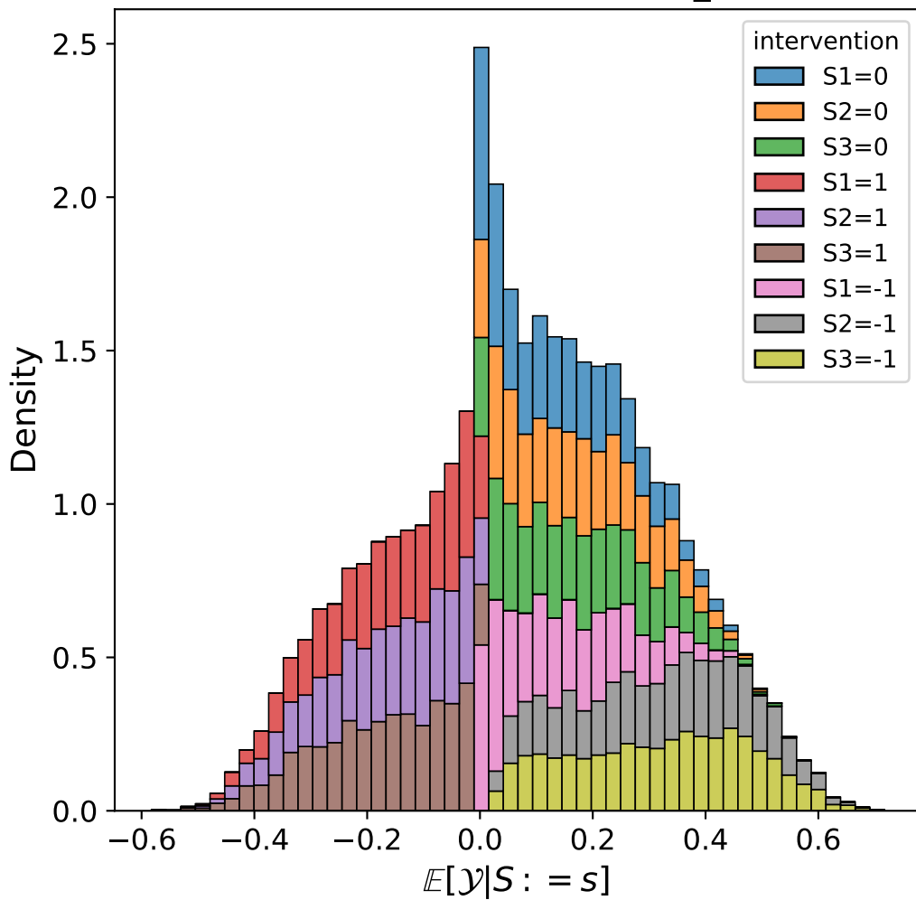
Variable y = Y1 , fold=k_2
