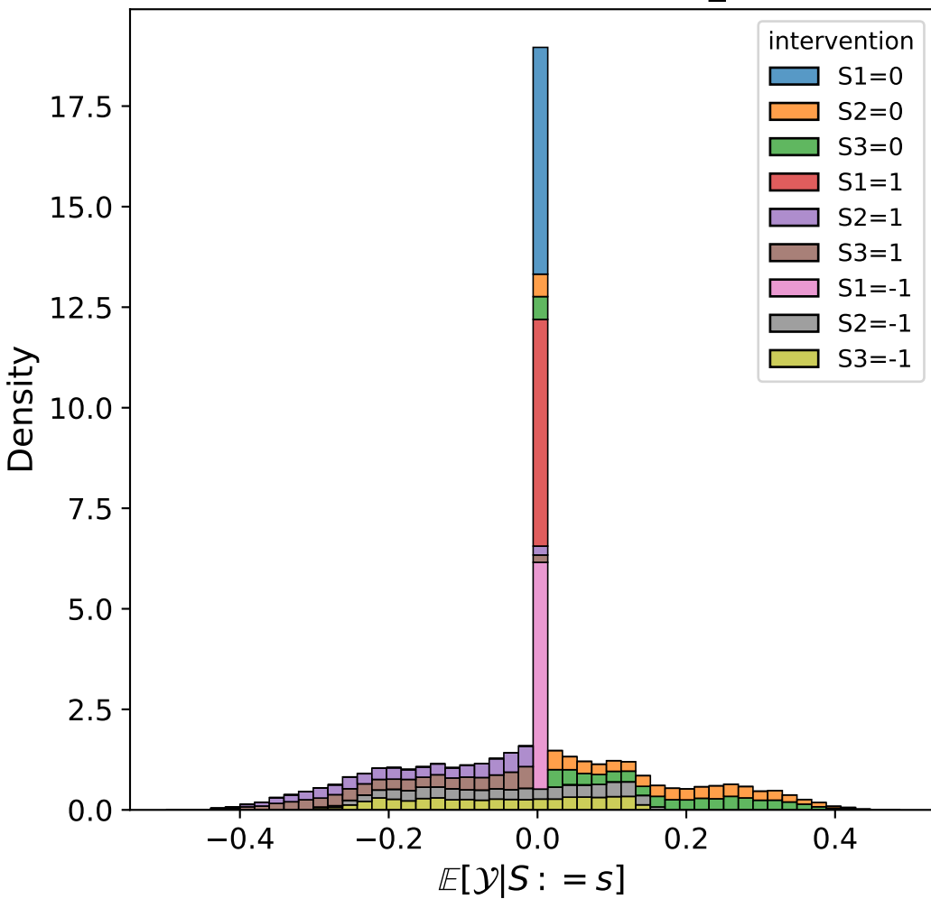
Variable y = Y2 , fold=k_4
