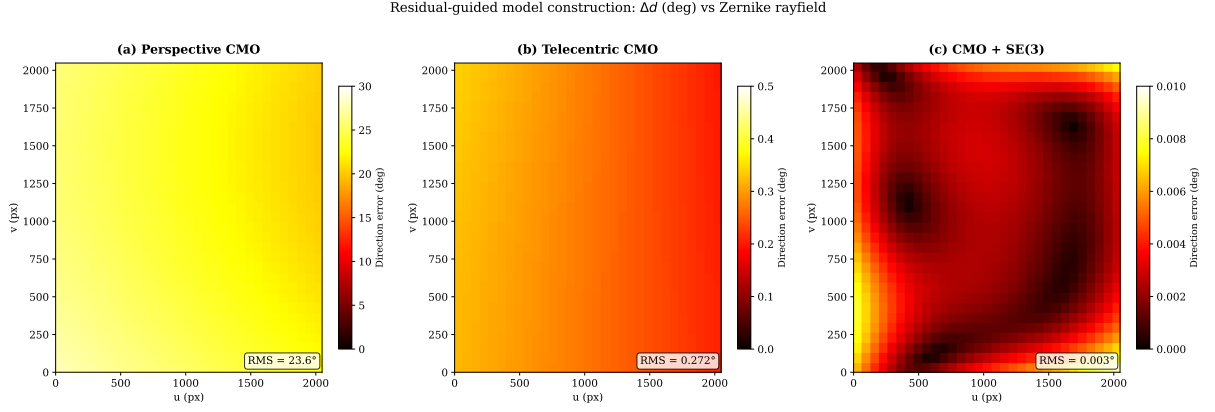
Figure 6. Residual evolution across model stages. Direction error \Delta d (degrees) between the Zernike rayfield (reference) and each candidate model, evaluated on a 31 \times 31 pixel grid. Left: Perspective CMO — large structured error (RMS 23.6^\circ , max 27.7^\circ ), dominated by a strong d_y gradient. Centre: Telecentric CMO — RMS drops to 0.27^\circ (two orders of magnitude), but the residual is still Z_0^0 -dominated (global piston), revealing the missing SE(3) arm alignment. Right: CMO + SE(3) — RMS drops to 0.003^\circ , near the noise floor. The residual heatmap at each stage directly tells the user what is wrong and where to look next.
