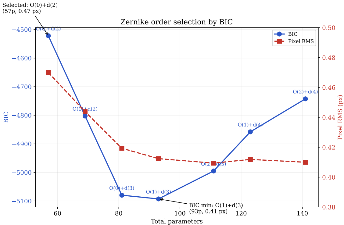
Figure 3. Zernike order exploration by BIC. Pixel RMS falls from 0.47 px at 57 params to 0.41 px near the BIC minimum (93 params) and then saturates (it is not strictly monotonic beyond, varying by < 0.005 px up to 141 params), but BIC penalises complexity. The BIC minimum is at \text{O}(1)+\text{d}(3) (93 params, \text{BIC} = -5093 , \text{RMS} = 0.41 px), while \text{O}(0)+\text{d}(2) (57 params, \text{BIC} = -4522 ) is within \sim 10\% in RMS at 40 % fewer parameters. The \text{O}(0)+\text{d}(2) model (57 params, 0.47 px) is retained as a deliberately constrained central-reference rayfield for compact CMO model construction, not as the statistical optimum.
