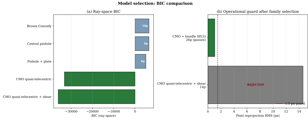
Figure 12. Two-panel BIC bar chart. (a) Ray-space BIC: the quasi-teletentric CMO family achieves the lowest BIC by a decisive margin over the non-CMO alternatives ( > 40\,000 points). (b) Operational usability guard with a 1.5 px reprojection threshold: models exceeding the threshold are marked as REJECTED (shown in grey/orange); only the 26p SE(3)-aligned model passes the guard (shown in green).
