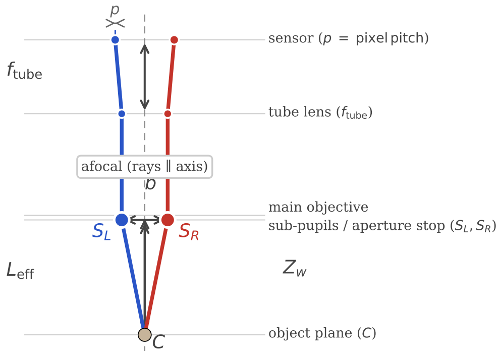
Figure 1. Effective first-order chief-ray skeleton for a CMO stereo microscope, not a literal lens layout. Two off-axis sub-pupils share a single main objective and feed two parallel stereo channels; the compact model represents the measured rays by effective sub-pupil locations, chief-ray directions, pupil shear, and per-channel bundle alignment.
