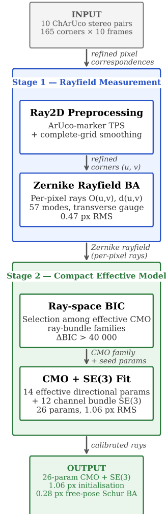
Figure 2. Pipeline overview. The two-stage decomposition separates rayfield measurement (Ray2D preprocessing + Zernike BA) from compact effective-model identification (ray-space BIC selection). The Ray2D stage is purely 2D and does not impose a 3D camera model.
