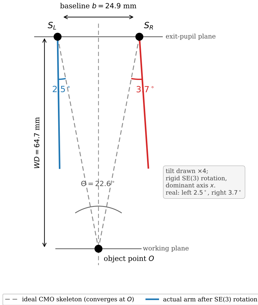
Figure 6. Per-channel SE(3) bundle alignment (schematic). The ideal quasi-telecentric CMO skeleton (dashed) places two off-axis effective sub-pupils S_L, S_R on the baseline b , emitting chief rays that converge on the optical axis at the object point O at working distance WD with full convergence angle \Theta . The fitted rigid SE(3) rotation tilts each effective ray bundle away from this ideal by \sim 2.5^\circ (left) and \sim 3.7^\circ (right); the tilt is drawn \times 4 for visibility. The rotation is a rigid SE(3) of the whole ray bundle, dominated by its x -component (fitted per-axis values: left (-2.3, -0.7, 0.6)^\circ , right (-2.6, -2.7, 0.2)^\circ ). These rotations are equivalent bundle-alignment parameters, not a unique mechanical diagnosis.
