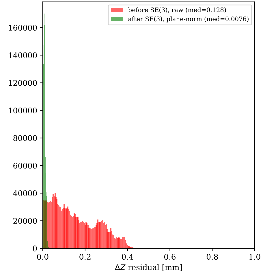
\Delta Z plane-norm: 0.0076 mm; 3D p2p: 3.5 \rightarrow 0.019 mm
