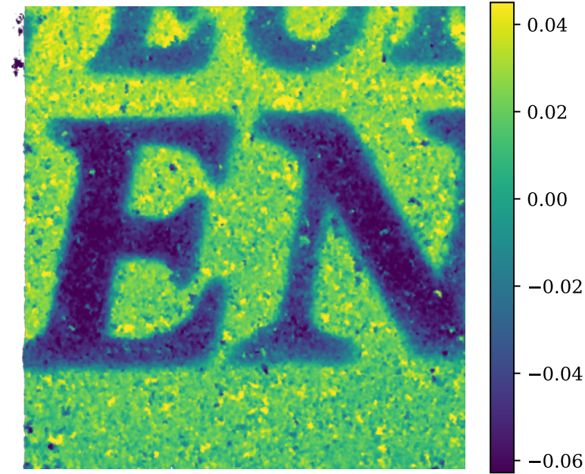
Zernike 57p Z (SE3+plane-norm) std=0.0315 mm
