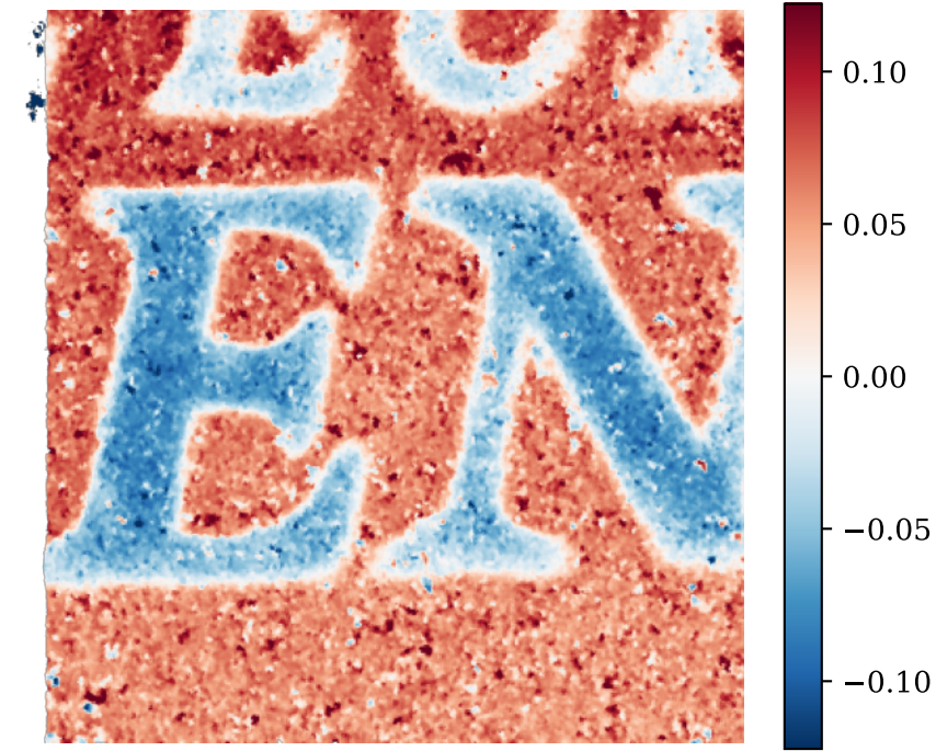
dZ after SE(3) med=0.055 mm
