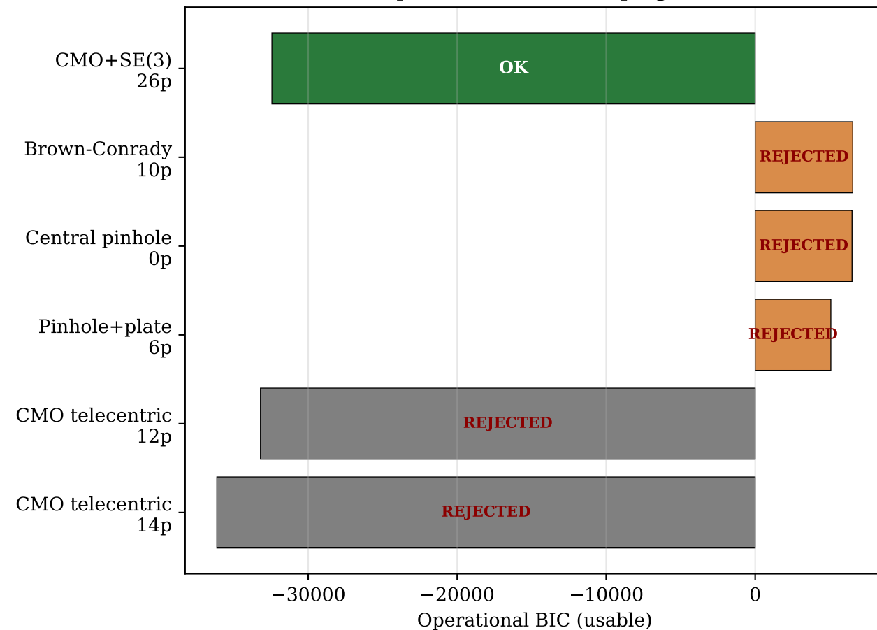
(b) Operational BIC (1.5 px guard)
