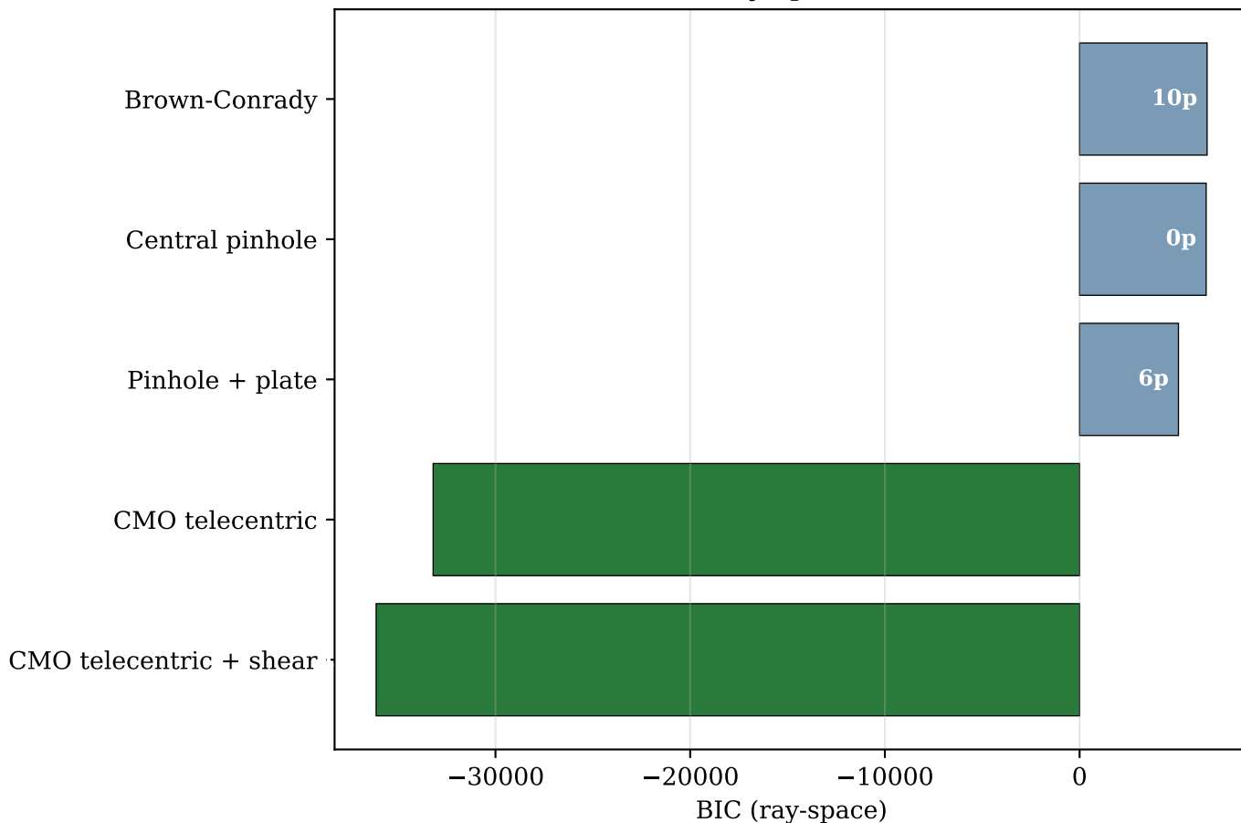
(a) Ray-space BIC
