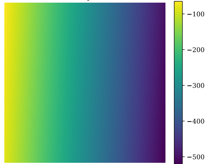
Affine plane
