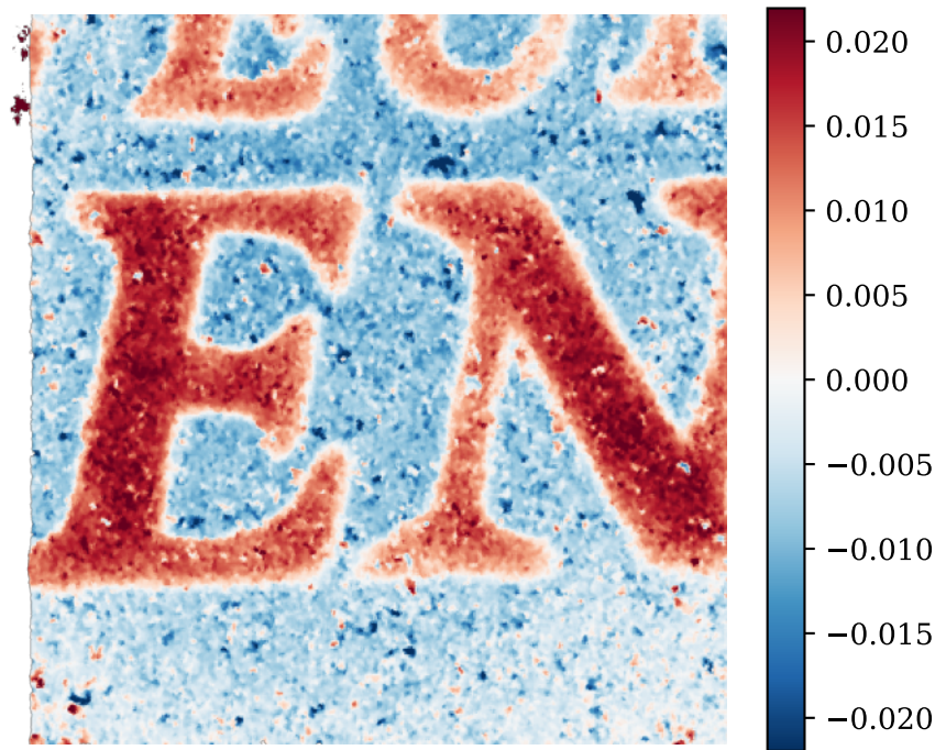
dZ plane-norm med=0.0076 mm
