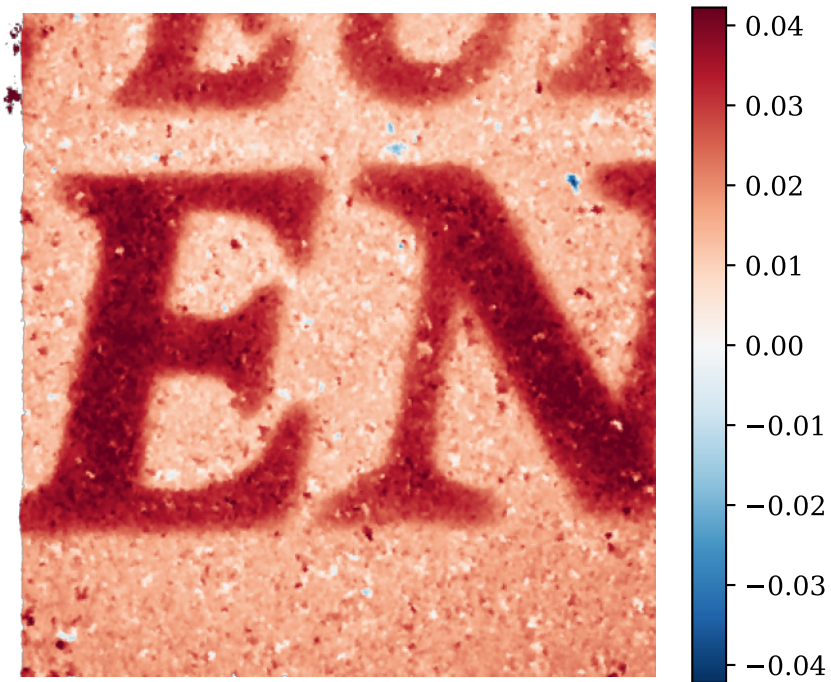
dZ after SE(3) med=0.018 mm
