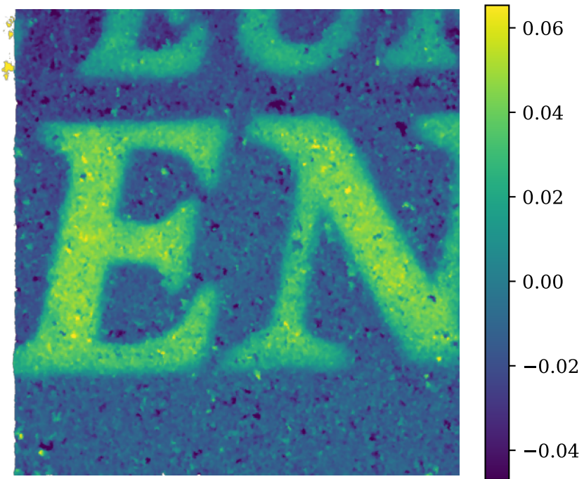
CMO 26p Z (plane-norm) std=0.0229 mm
