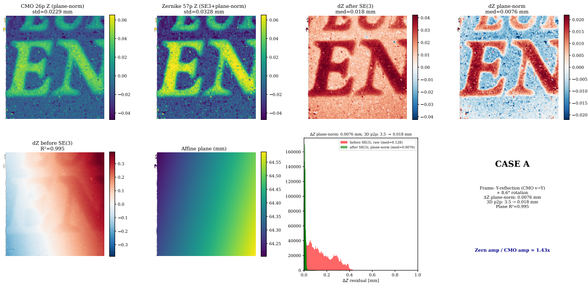
Figure 10. Rigid-gauge removal: Zernike vs CMO surface comparison. Top row: CMO and Zernike surfaces after plane-normalisation (relief only), followed by \Delta Z before and after plane normalisation. Bottom row: \Delta Z before SE(3) alignment (dominated by an affine ramp, R^2 = 0.995 ), the fitted affine plane, and the residual histogram. After SE(3) alignment the median plane-normalised \Delta Z residual is 0.0076 mm; the corresponding median 3D point-to-point residual drops from 3.5 mm to 0.018 mm (a 99.5 % reduction). The remaining relief difference is a depth-only scalar (relief-amplitude ratio Z_{\text{Zernike}}/Z_{\text{CMO}} = 1.43\times , i.e. s_z \approx 0.70 ): the two reconstructions agree up to a single depth-scale factor, not a spatially arbitrary non-rigid discrepancy. Which reconstruction is closer to the true surface requires an external axial reference (§5.2).
