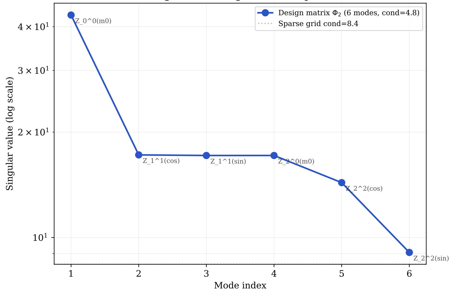
Design matrix singular value spectra
