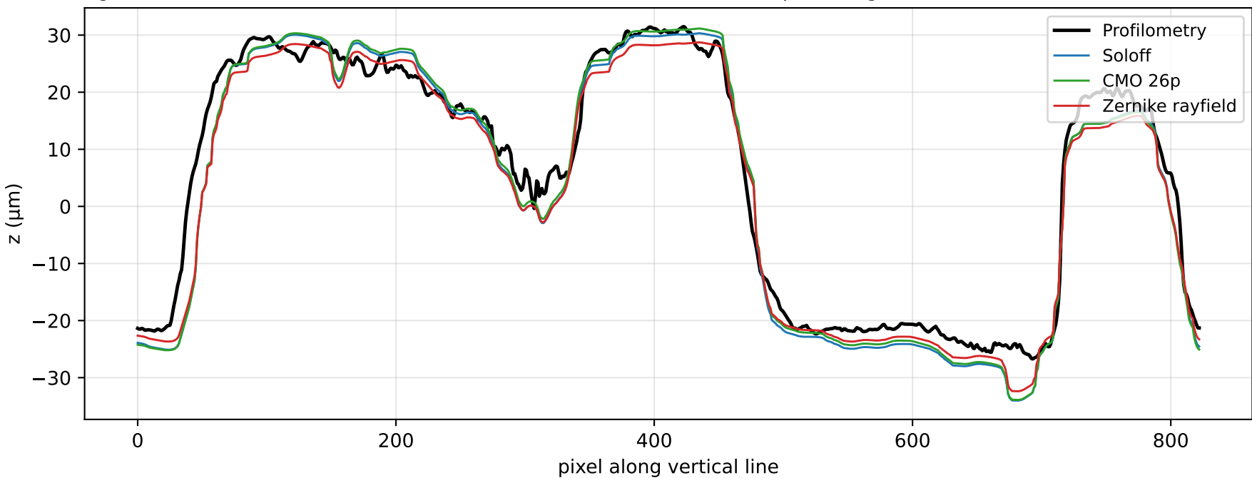
(e) z along the vertical line — Soloff and CMO coincide (cc=1.000, RMS=0.56 \mu\text{m} ); stage-anchored Zernike recovers the metric relief
