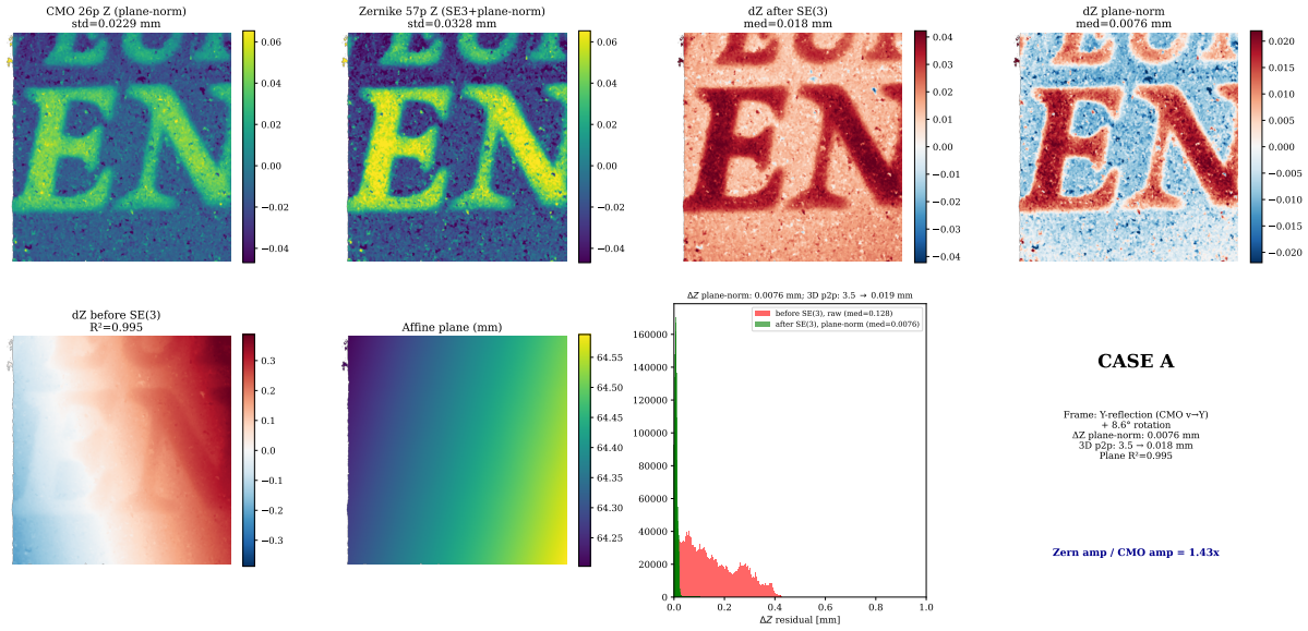
Figure 10. Rigid-gauge removal: Zernike vs CMO surface comparison. Top row: CMO and Zernike surfaces after plane-normalisation (relief only). \Delta Z raw and plane-normalised residuals. Bottom row: \Delta Z before SE(3) alignment (dominated by an affine ramp, R^2 = 0.995 ), the fitted affine plane, and the residual histogram. After SE(3) alignment the two relief maps agree to a median plane-normalised \Delta Z residual of 0.0076 mm (the principal relief-comparison metric); the corresponding median 3D point-to-point residual drops from 3.5 mm to 0.018 mm (a 99.5 % reduction). The interpretation is Case A: the Zernike and CMO reconstructions differ by the CMO model’s v \rightarrow Y sign convention (a Y-axis reflection) plus a small ( \sim 8.6^\circ ) rigid rotation, not by a genuine non-rigid rayfield discrepancy. Once the reflection is removed the two relief maps agree in sign.
