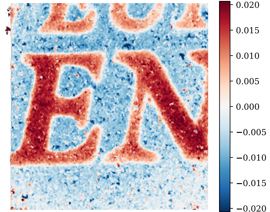
dZ plane-norm med=0.007 mm
