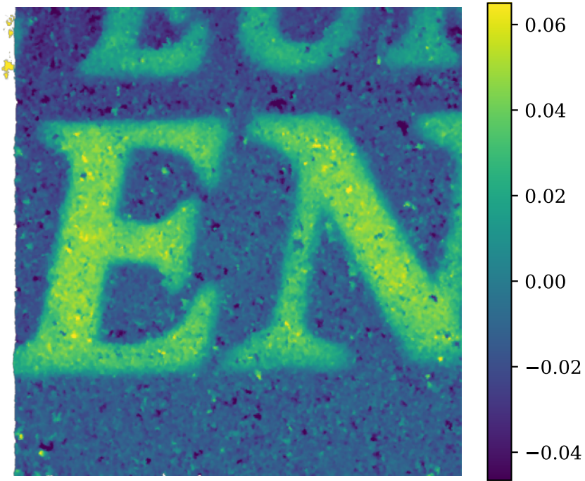
CMO 26p Z (plane-norm) std=0.0235 mm
