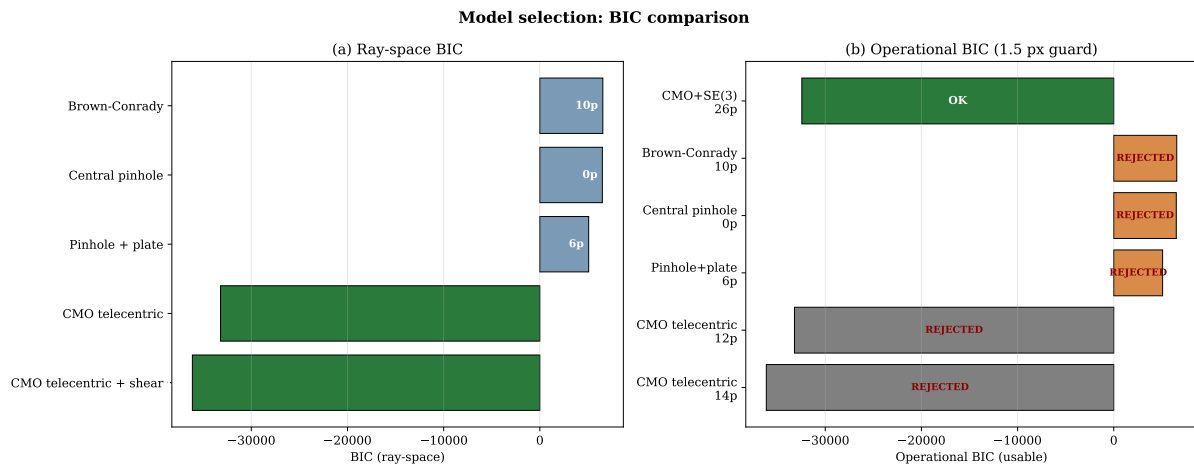
Figure 11. Two-panel BIC bar chart. (a) Ray-space BIC: the CMO telecentric family achieves the lowest BIC by a decisive margin (> 40 000 points). (b) Operational usability score with a 1.5 px reprojection guard: models exceeding the threshold are marked as REJECTED (shown in grey/orange); only the 26p SE(3)-aligned model passes the guard (shown in green).
