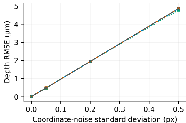
Fine sweep (0.08 mm)
