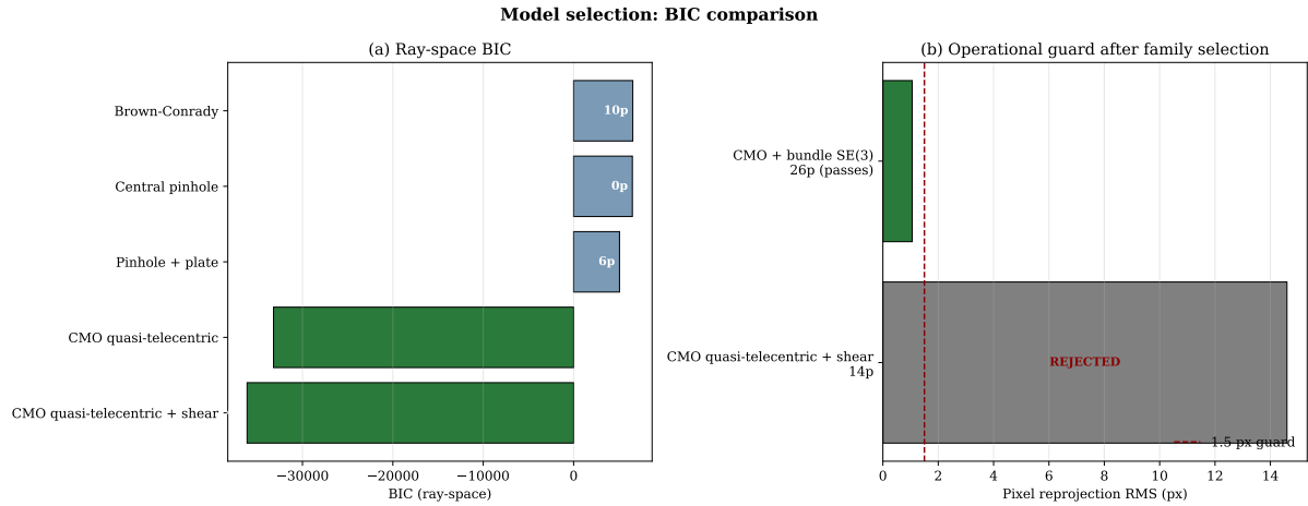
Figure 12. Two-panel BIC bar chart. (a) Ray-space BIC: the quasi-telecentric CMO family achieves the lowest BIC by a decisive margin over the non-CMO alternatives ( > 40\,000 points). (b) Operational usability guard with a 1.5 px reprojection threshold: models exceeding the threshold are marked as REJECTED (shown in grey/orange); only the 26p SE(3)-aligned model passes the guard (shown in green).
