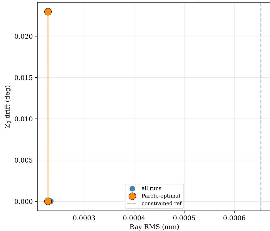
Pareto frontier: RMS vs gauge drift
