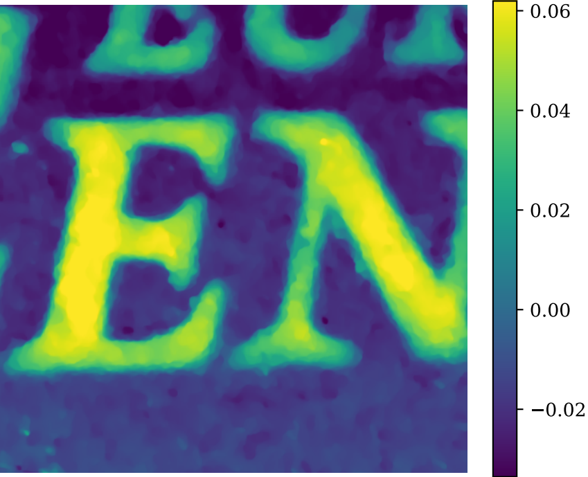
Zernike 57p Z (SE3+plane-norm) std=0.0287 mm
