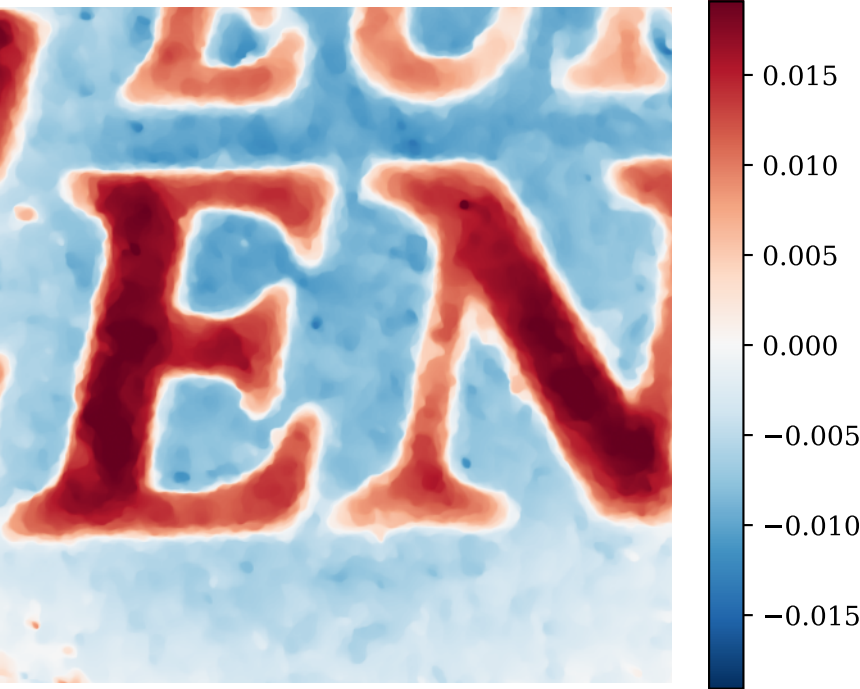
dZ plane-norm med=0.0070 mm
