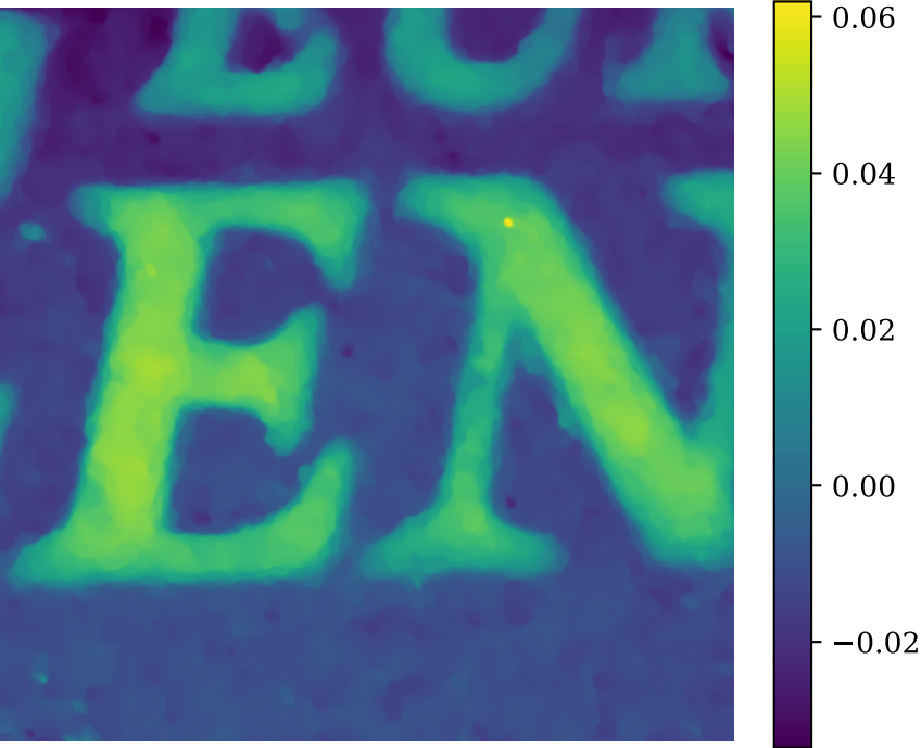
CMO 26p Z (plane-norm) std=0.0202 mm
