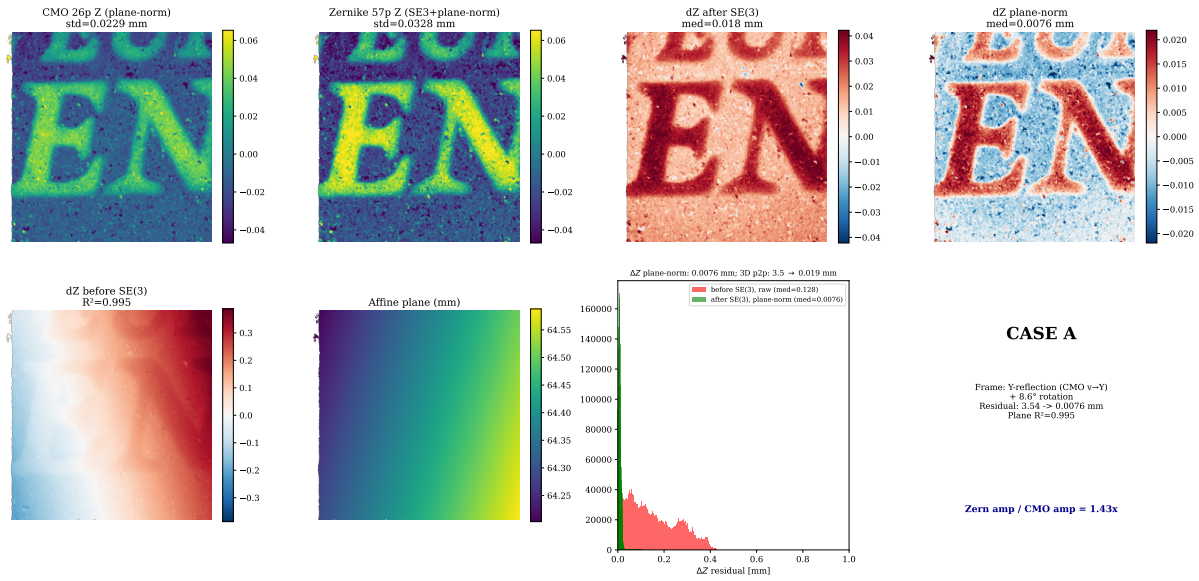
Figure 10. Rigid-gauge removal: Zernike vs CMO surface comparison. Top row: CMO and Zernike surfaces after plane-normalization (relief only). \Delta Z raw and plane-normalized residuals. Bottom row: \Delta Z before SE(3) alignment (dominated by an affine ramp, R^2 = 0.995 ), the fitted affine plane, and the residual histogram. After SE(3) alignment the two relief maps agree to a median plane-normalised \Delta Z residual of 0.0076 mm (the principal relief-comparison metric); the corresponding median 3D point-to-point residual drops from 3.5 mm to 0.019 mm (a 99.5 % reduction). The interpretation is Case A: the Zernike and CMO reconstructions differ by the CMO model’s v \rightarrow Y sign convention (a Y-axis reflection) plus a small ( \sim 8.6^\circ ) rigid rotation, not by a genuine non-rigid rayfield discrepancy. Once the reflection is removed the two relief maps agree in sign.
