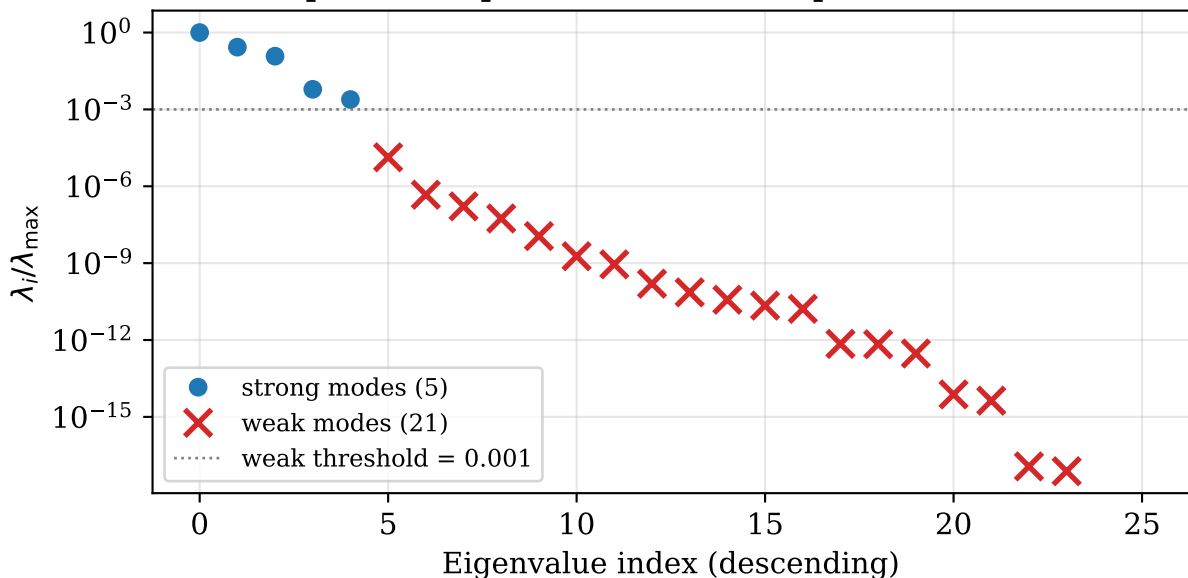
Schur complement spectrum of the 26-parameter CMO model
