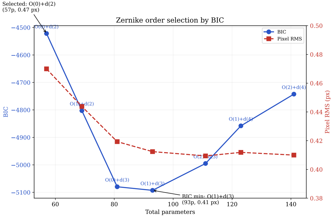
Figure 3. Zernike order exploration by BIC. Pixel RMS falls from 0.47 px at 57 params to 0.41 px near the BIC minimum (93 params) and then saturates (it is not strictly monotonic beyond, varying by < 0.005 px up to 141 params), but BIC penalises complexity. The BIC minimum is at \text{O}(1)+\text{d}(3) (93 params, \text{BIC} = -5093 , \text{RMS} = 0.41 px), while \text{O}(0)+\text{d}(2) (57 params, \text{BIC} = -4522 ) is within \sim 10\% in RMS at 40 % fewer parameters. The \text{O}(0)+\text{d}(2) model (57 params, 0.47 px) is retained as a deliberately constrained central-reference rayfield for compact CMO model construction, not as the statistical optimum.
