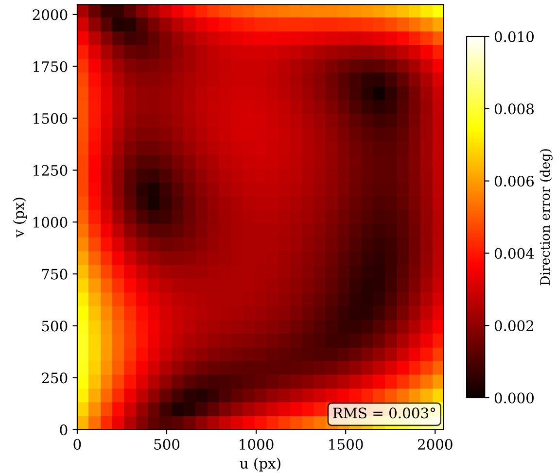
(c) CMO + SE(3)
