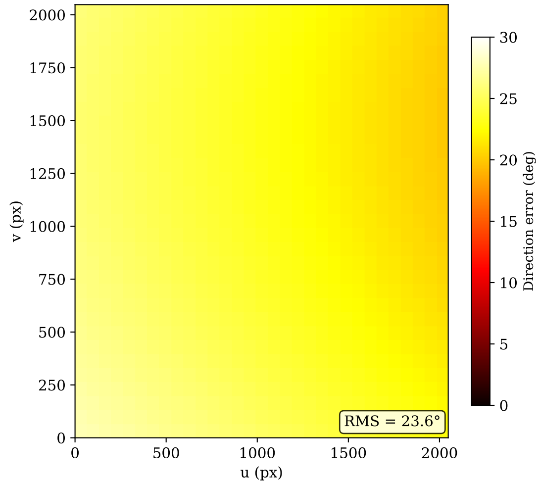
(a) Perspective CMO
