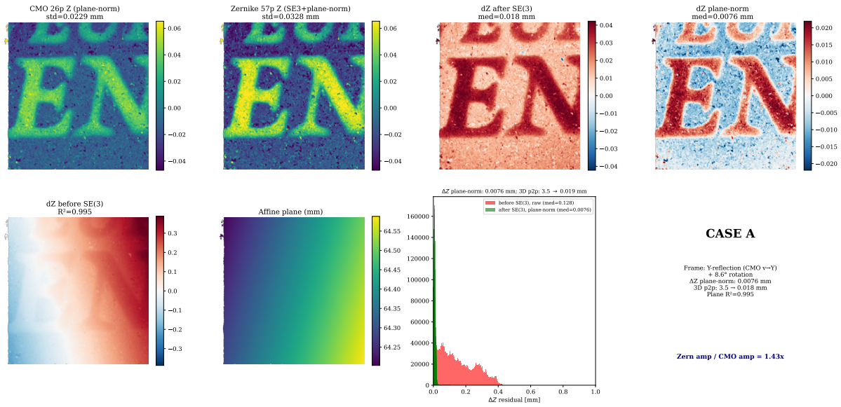
Figure 10. Rigid-gauge removal: Zernike vs CMO surface comparison. Top row: CMO and Zernike surfaces after plane-normalisation (relief only). \Delta Z raw and plane-normalised residuals. Bottom row: \Delta Z before SE(3) alignment (dominated by an affine ramp, R^2 = 0.995 ), the fitted affine plane, and the residual histogram. After SE(3) alignment the two relief maps agree to a median plane-normalised \Delta Z residual of 0.0076 mm (the principal relief-comparison metric); the corresponding median 3D point-to-point residual drops from 3.5 mm to 0.019 mm (a 99.5 % reduction). The interpretation is Case A: the Zernike and CMO reconstructions differ by the CMO model’s v \rightarrow Y sign convention (a Y-axis reflection) plus a small ( \sim 8.6^\circ ) rigid rotation, not by a genuine non-rigid rayfield discrepancy. Once the reflection is removed the two relief maps agree in sign.
