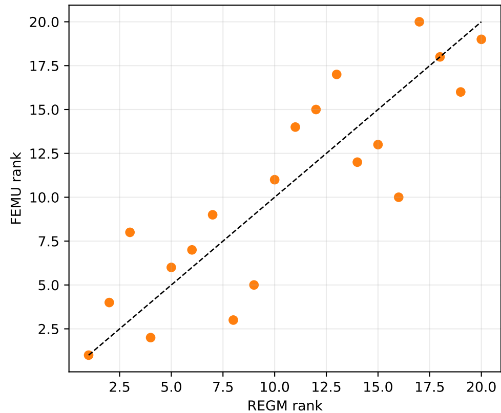
Preregistered M8 SRIX parameter-ranking gate
