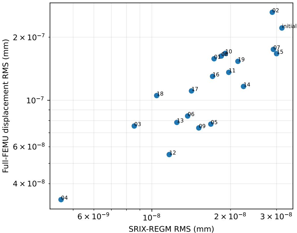
Preregistered M8 SRIX parameter-ranking gate
