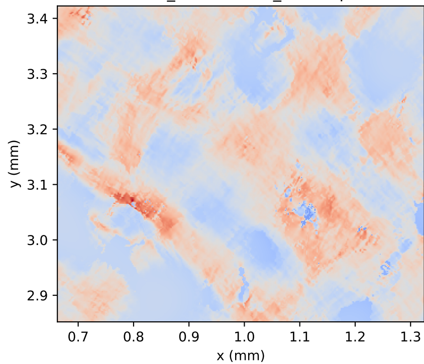
NONLOCAL_HARDENING_MPA, alpha = 4
