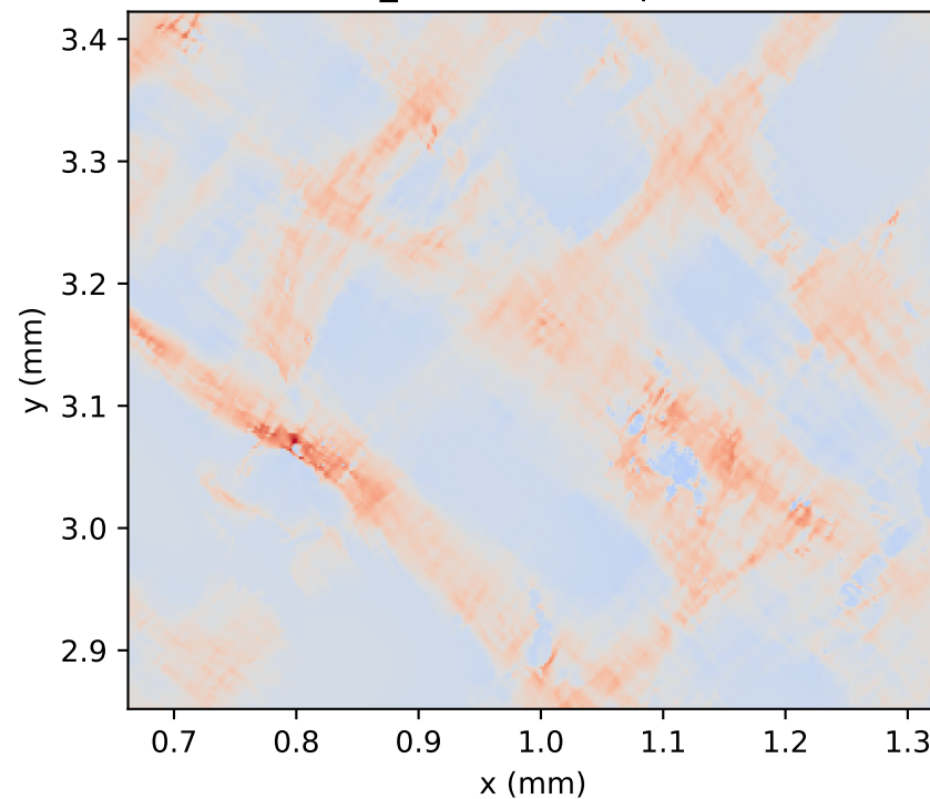
PEEQ_MISMATCH, \alpha = 4
