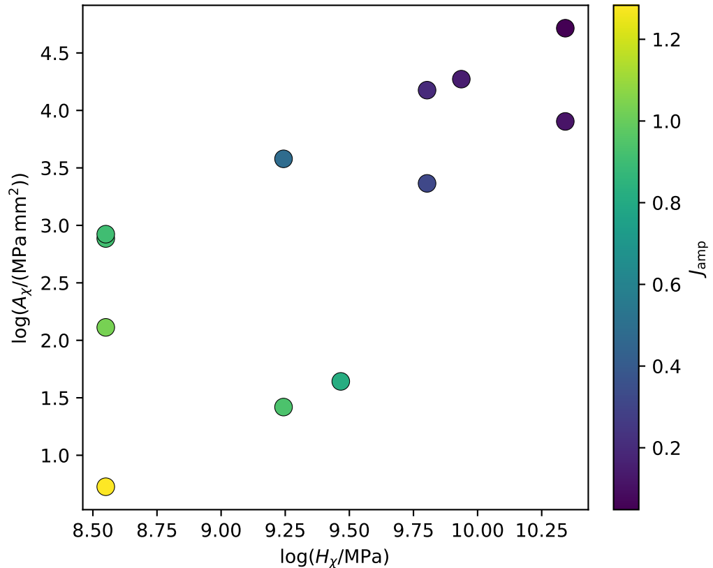
Identifiability coordinates
