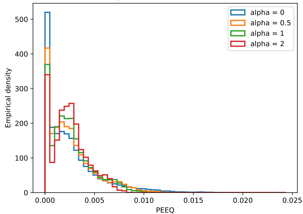
PEEQ distributions on P154 core
