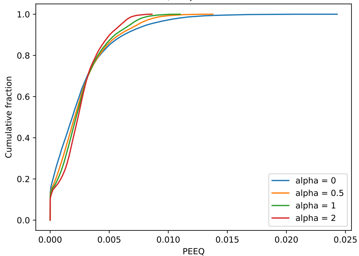
PEEQ empirical CDF
