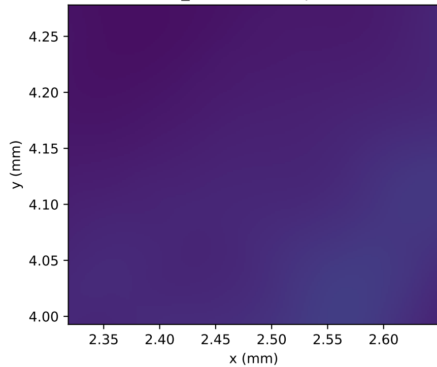
PEEQ_NONLOCAL, \alpha = 1
