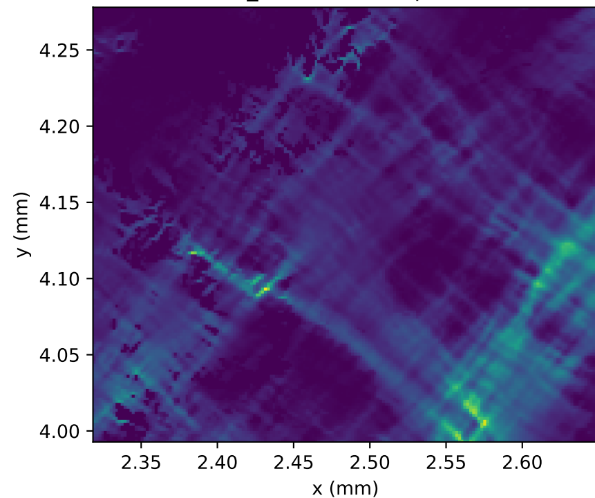
PEEQ_NONLOCAL, \alpha = 1
