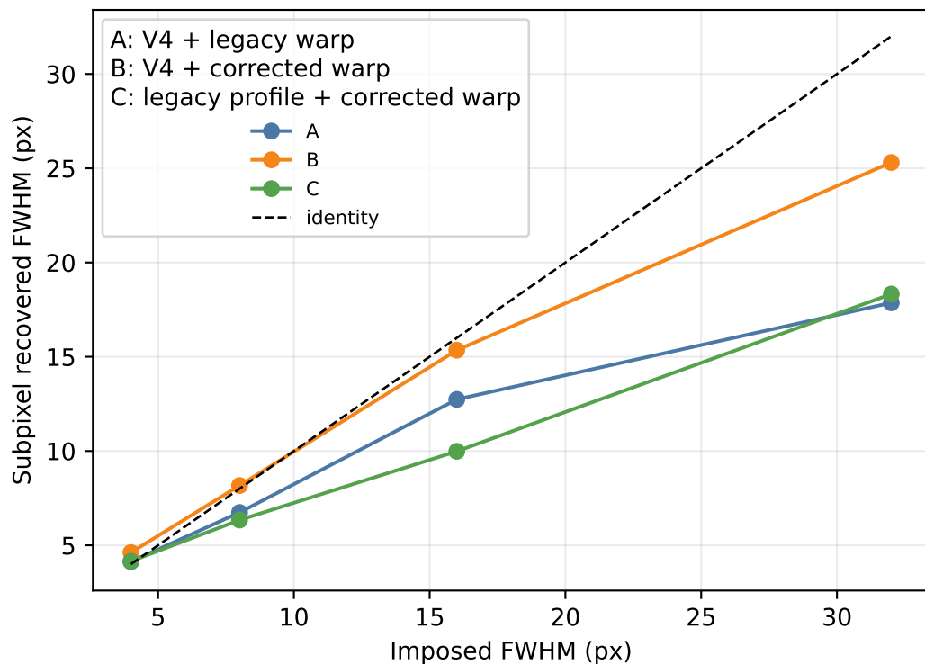
DISFlow profile and forward-warp sensitivity — horizontal bands
