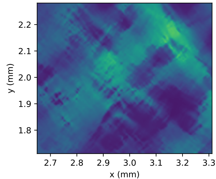
PEEQ, max=0.0090 band width=0.1061 mm
