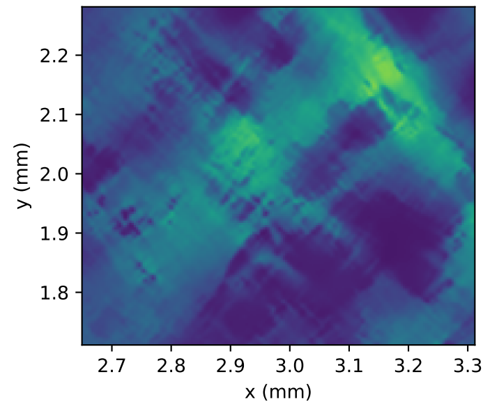
PEEQ, max=0.0097 band width=0.1159 mm
