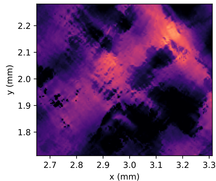
PEEQ, max=0.0097 band width=0.1159 mm
