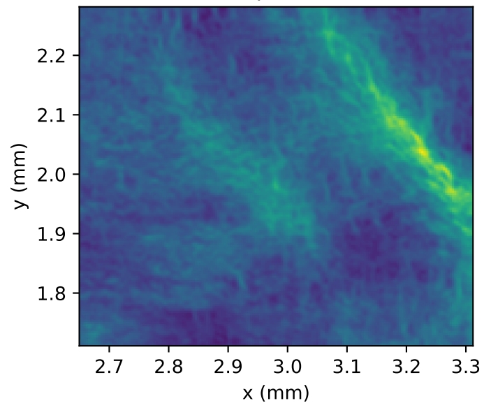
DIC total equivalent strain
