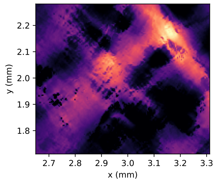
PEEQ, max=0.0120 band width=0.1248 mm
