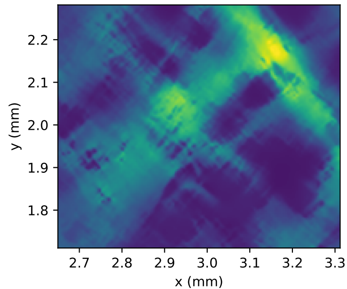
PEEQ, max=0.0120 band width=0.1248 mm
