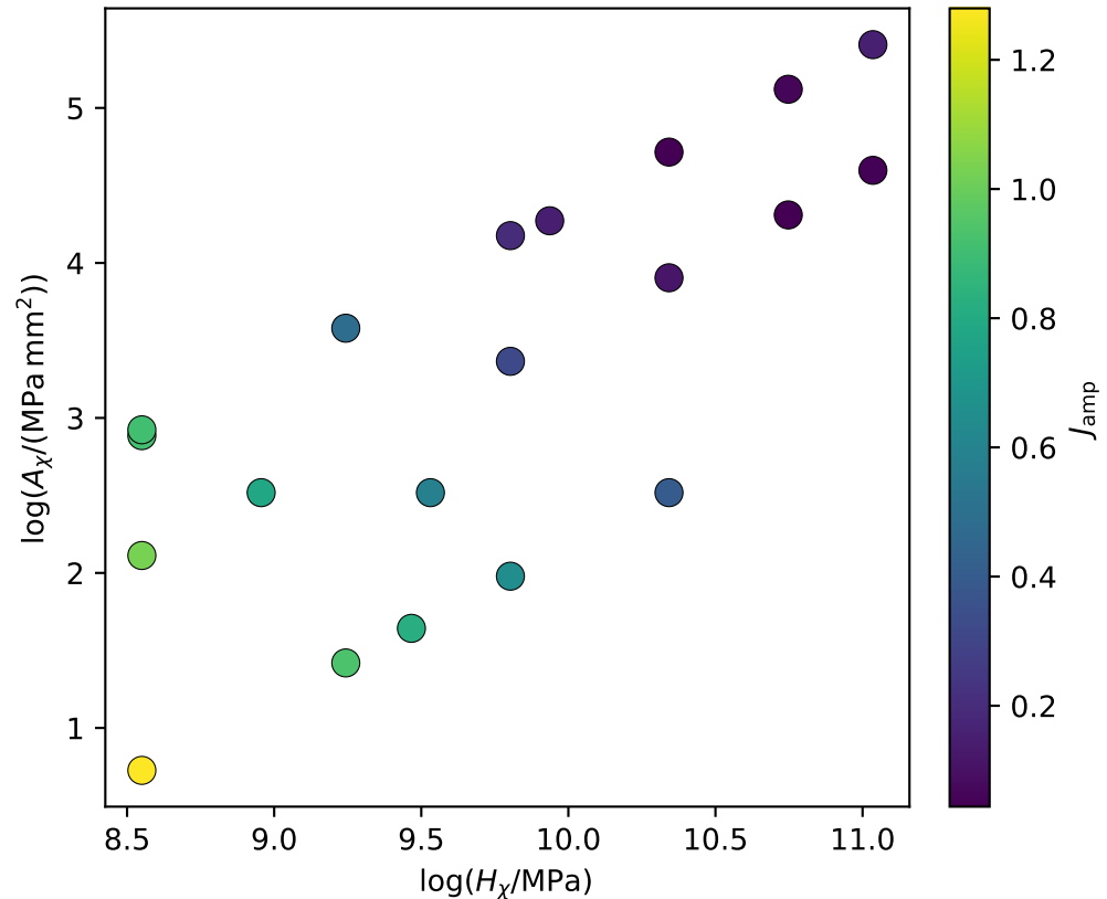
Identifiability coordinates
