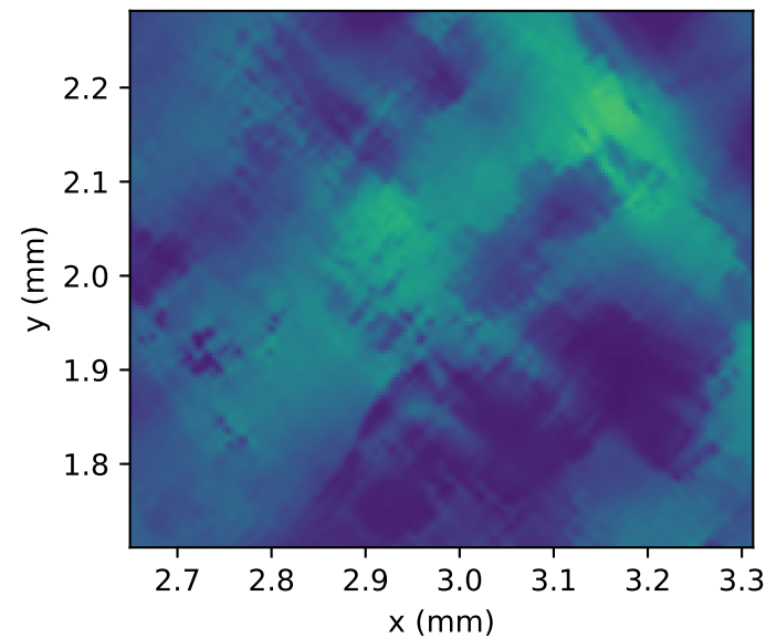
PEEQ, max=0.0081 band width=0.1096 mm
