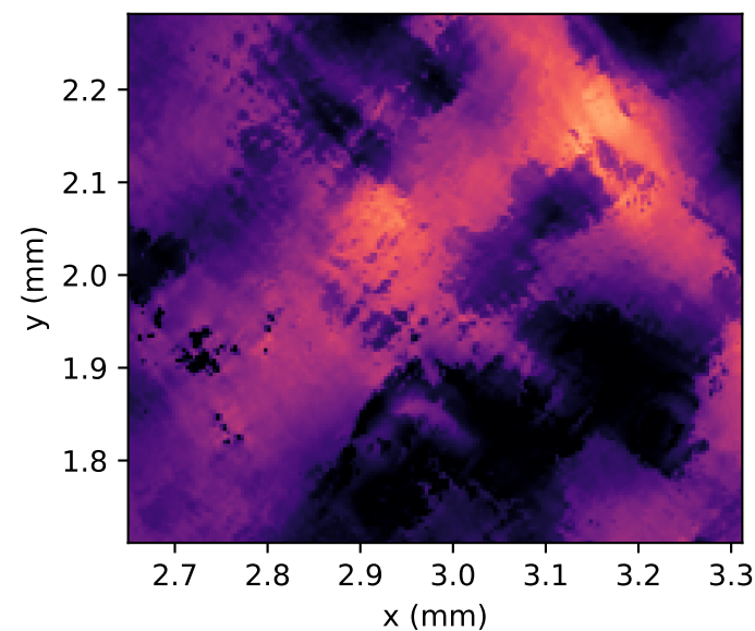
PEEQ, max=0.0081 band width=0.1096 mm
