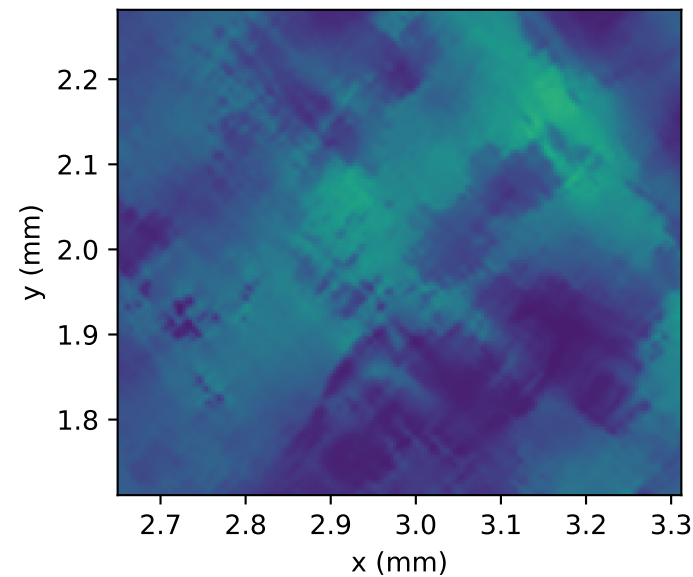
PEEQ, max=0.0073 band width=0.0617 mm
