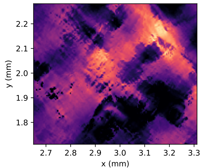
PEEQ, max=0.0090 band width=0.1061 mm
