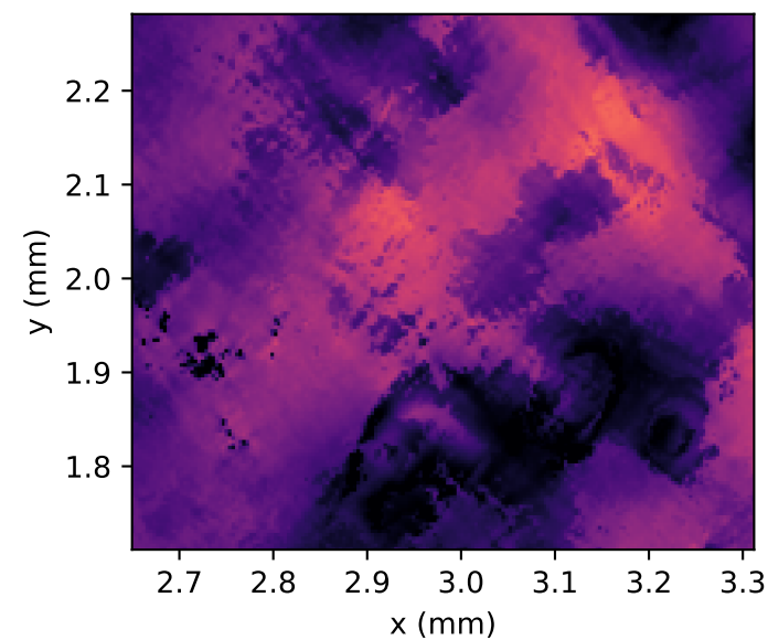
PEEQ, max=0.0064 band width=0.0525 mm
