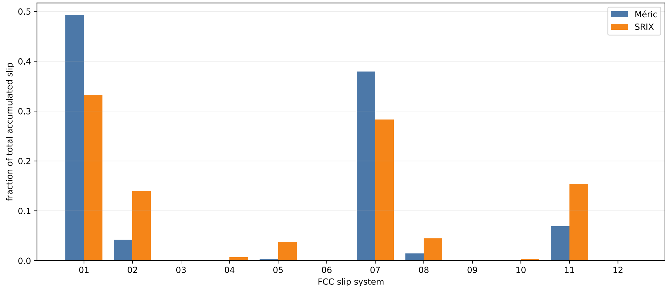
Per-system contributions — S95 Jaccard=0.800, TV=0.256, rank rho=0.9384571137702377
