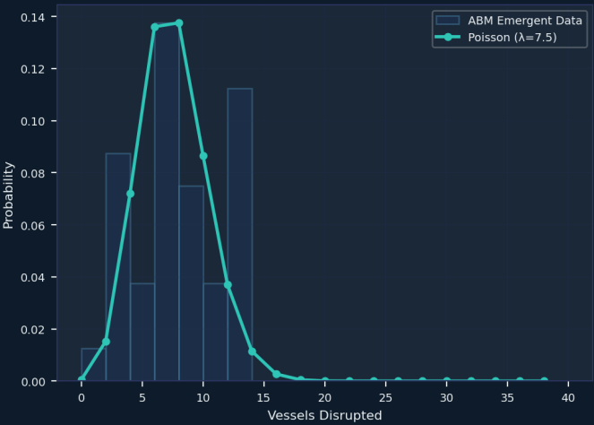
Queuing Theory – Arrival Rate Fit
