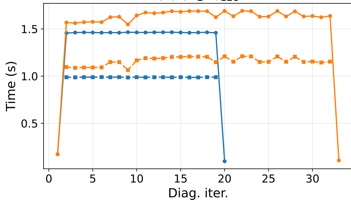
(c) \text{MAPbI}_3
