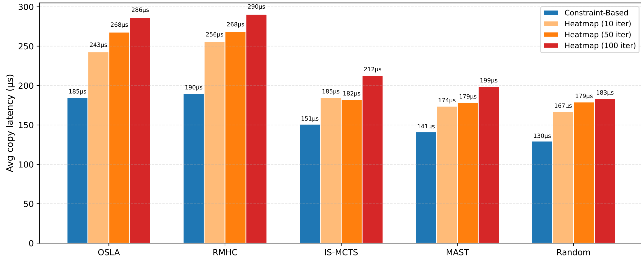
Average copy latency per agent Constraint-Based vs Heatmap-Guided (10/50/100 iter)
