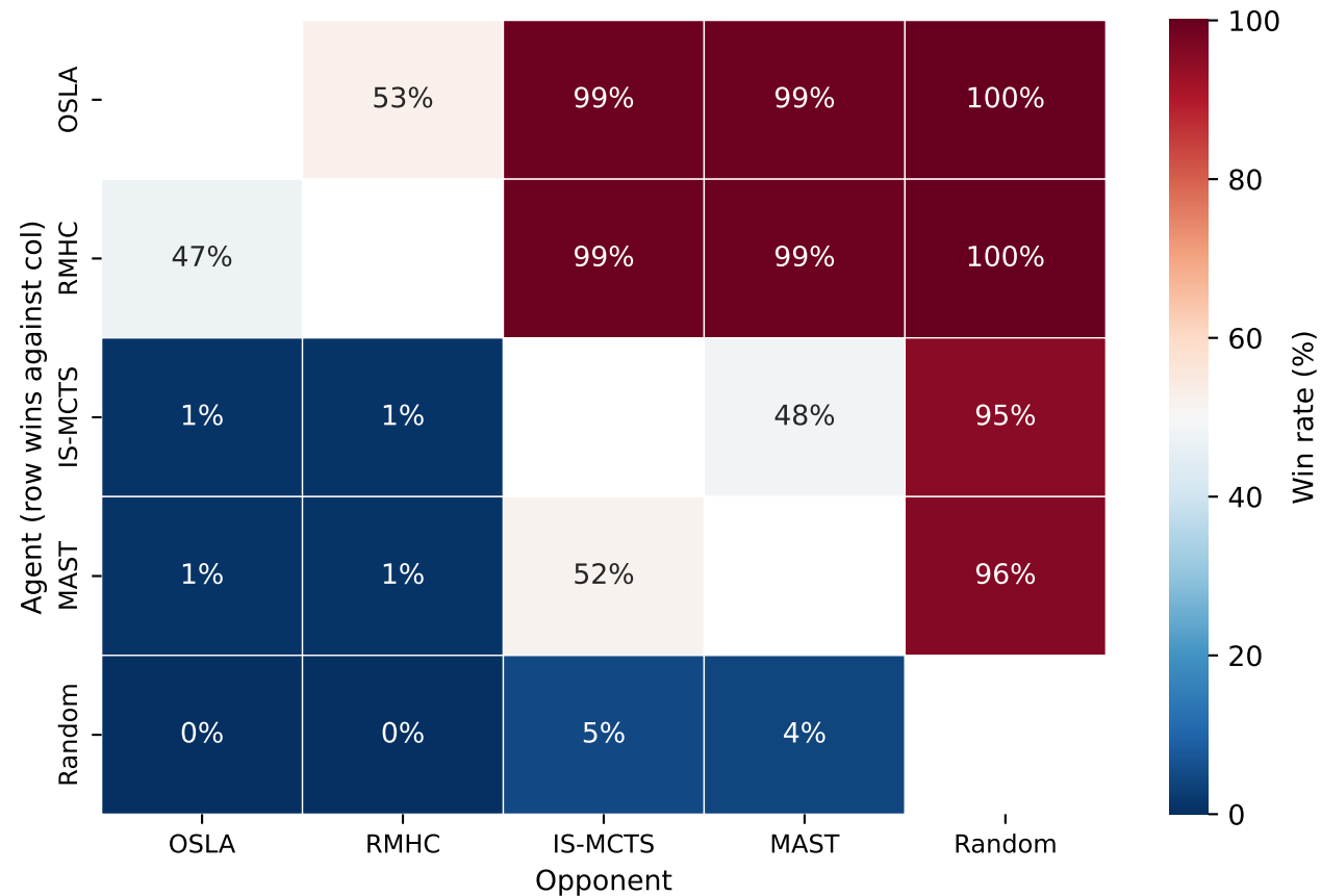
Head-to-head - Constraint-Based Det.
