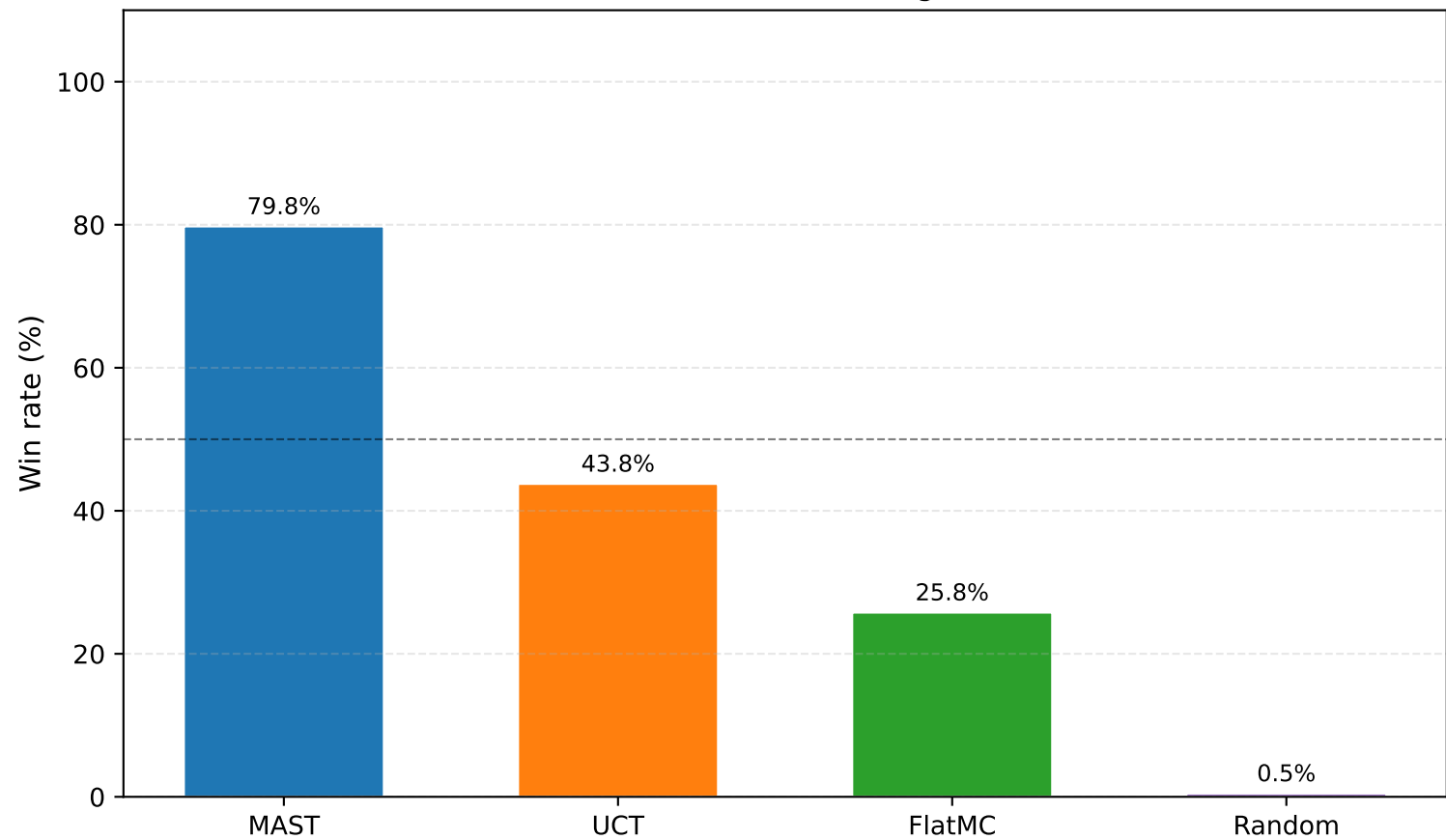
Tournament 1 (native agents)
