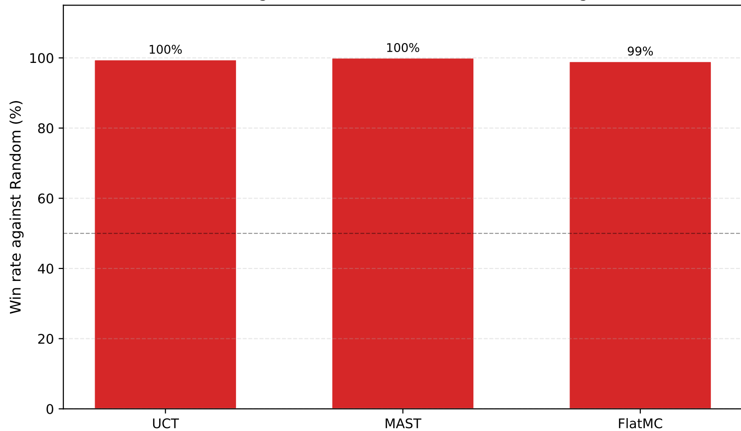
Win rate against Random - Tournament 1 (native agents)
